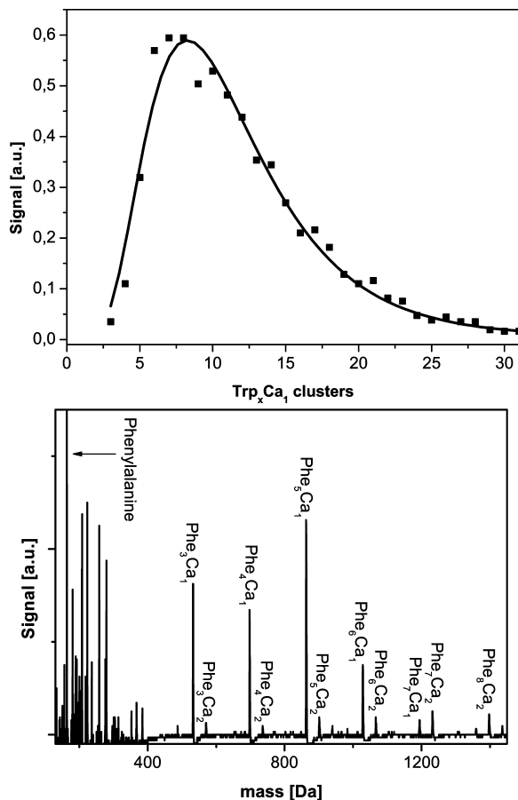
Figure 7. Neutral metal–organic complexes form after laser desorption from a mixture of amino acid powder with a metal salt and cellulose. Top: Cluster distribution of \text{Trp}_x\text{Ca}_1 resulting from desorbed tryptophan and \text{CaCO}_3 fitted with a log-normal distribution. Ionization of the clusters was done with VUV light, and argon was used as seed gas. 26 Bottom: Phenylalanine and \text{CaCO}_3 ionized with UV radiation (backing gas: argon).
